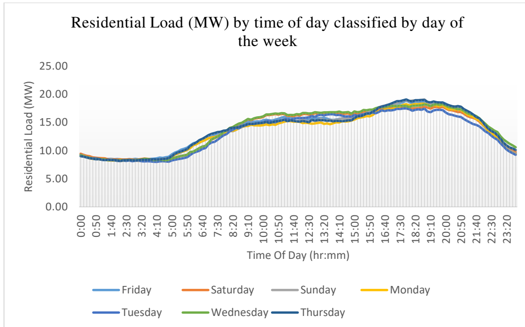
Figure 1: Residential Load Curves by time of day and day of the week (no EV charging)
