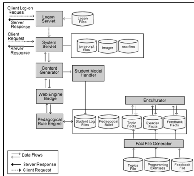
Figure 1. Enculturated web-based ITS system architecture
