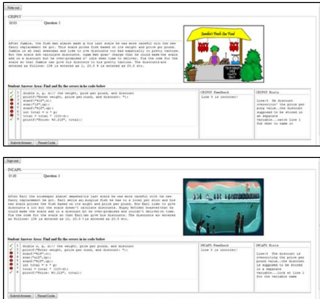
Figure 2. Screenshots of CRIPSY (top) and INCAPS (bottom) featuring enculturated and non-cultural versions of the same programming exercise.
