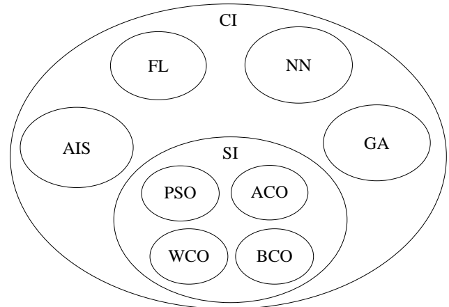
Fig. 1: CI techniques
