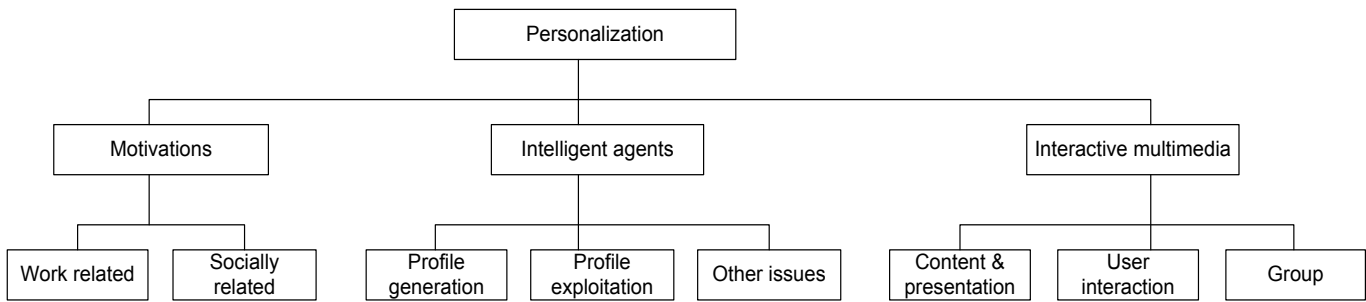
Fig. 9 Personalization taxonomies
