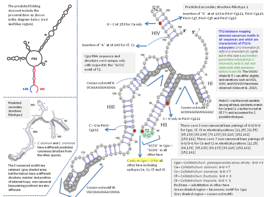
Figure 6 Consensus secondary structure of the ITS2 marker mapped onto C. gloeosporioides sensu stricto (type sequence EU371022) whose structure was retrieved from the ITS2 database.
