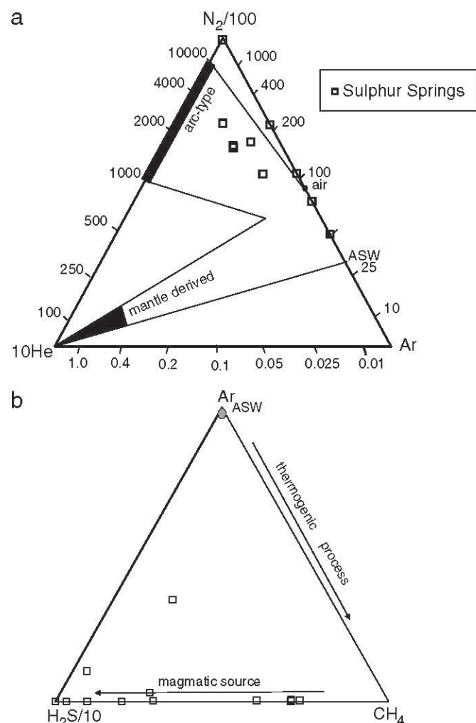
Fig. 8. (a) Ar–N 2 –He and (b) CH 4 –Ar–H 2 S ternary diagrams for hydrothermal gases of Sulphur Springs.
