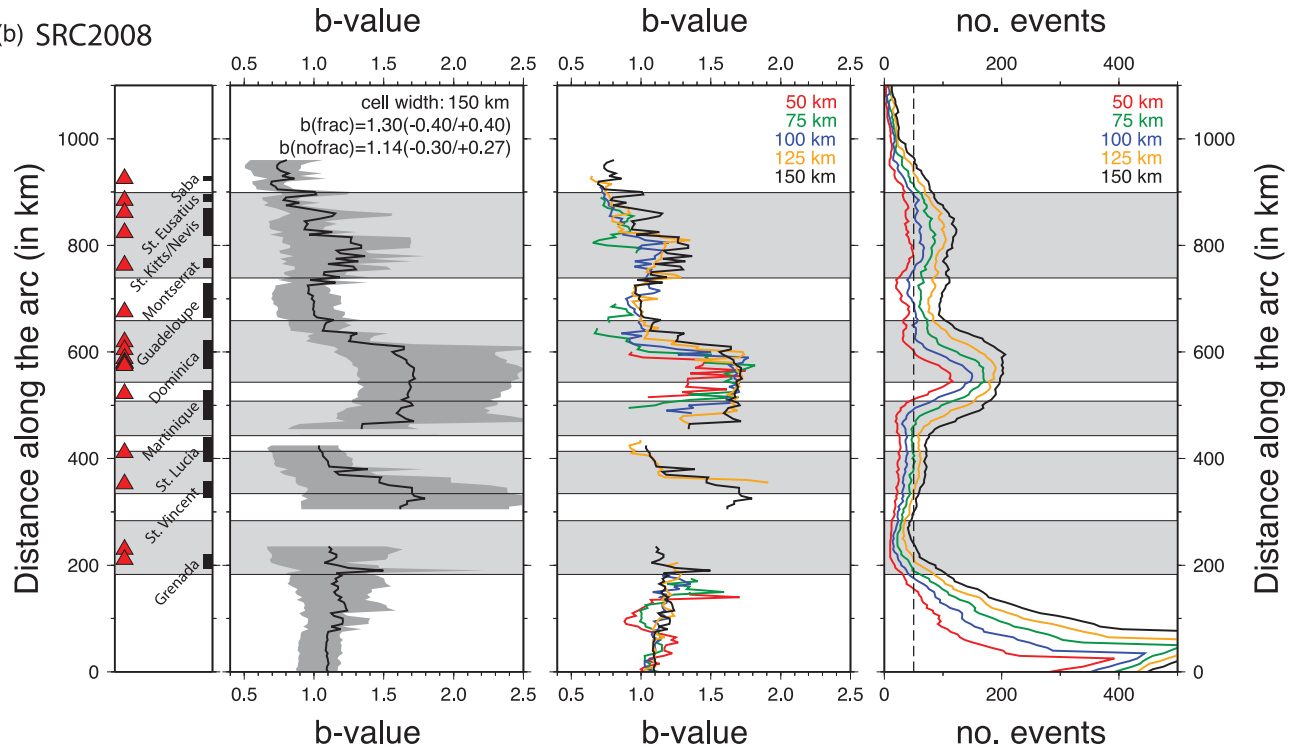
Figure 8. Results for the along-arc observation using fixed cell sizes. The observation was done using OVS1996 (a) and SRC2008 (b). Column 1 (subimage on the left-hand side): Positions of volcanoes (red triangles) and islands (black rectangles) along the arc. The horizontal areas in grey represent the areas around the subducted fracture zones including the associated core complexes. Column 2: Calculated b -values for one cell width with its uncertainties. The average b -values in areas where of subducted fracture zones and the remaining areas are calculated using all results in the grey shaded areas ('frac') and the white gaps ('nofrac'). Note the change of the b -value upper limit between the two catalogues. Column 3: Results without uncertainties for a range of different cell widths. Note that the range of values is generally less than the calculated uncertainties for a single cell size. This implies that cell size is not a critical parameter in this study. Column 4: Number of events per cell. The dashed black line shows the minimum required number for the b -value calculation (50). Note that there is no set maximum number of events per cell; we only cut the figure at 500 events per cell for clarity.
