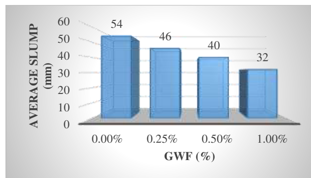
Figure 3: Slump test results of fresh concrete mixes
