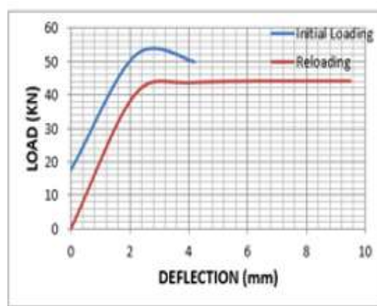
Figure 11: Initial load/Reloading load-deflection response curve (0.50% GWF with SR)
