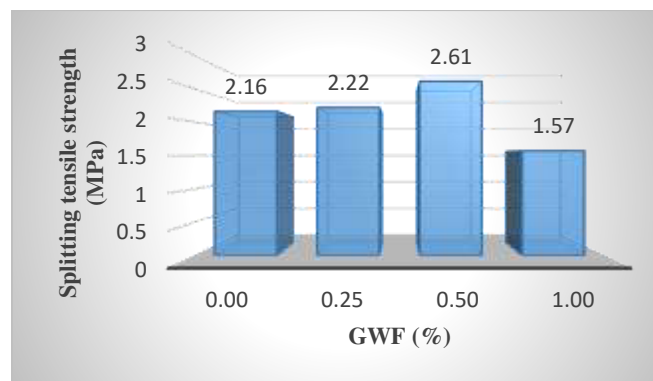
Figure 5: Splitting tensile strength vs. GWF (%)
