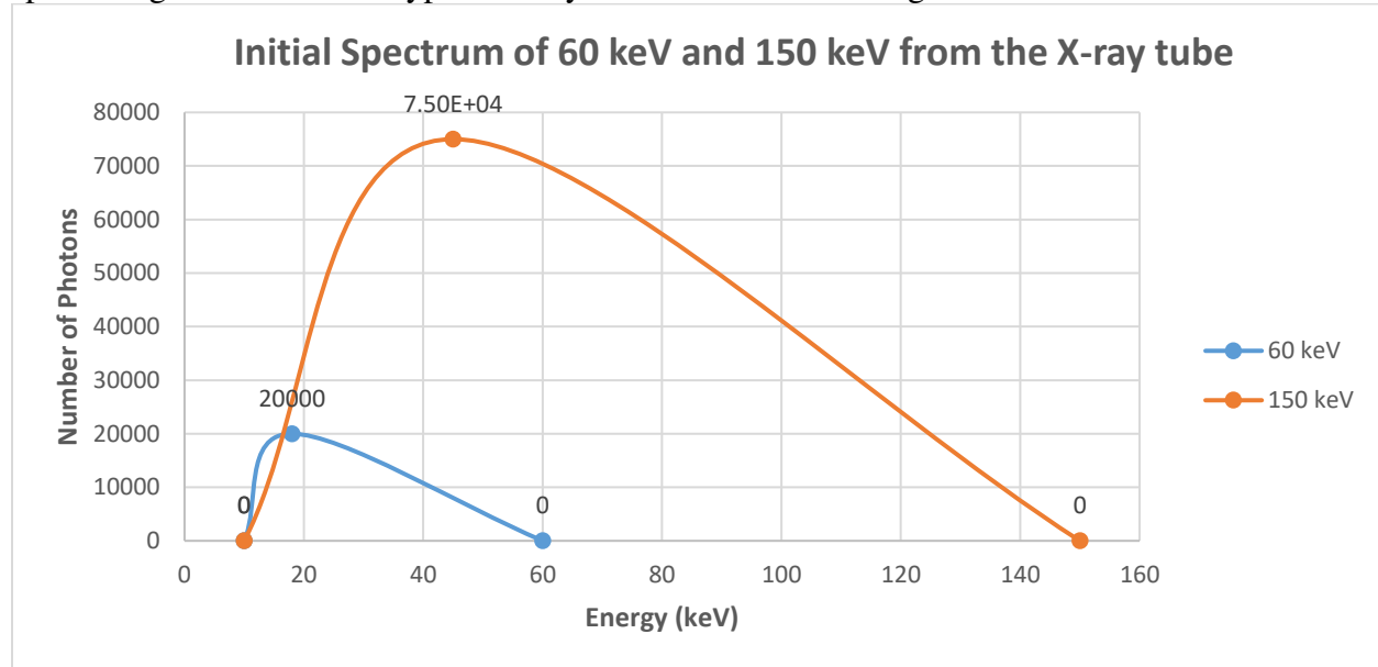
Figure 2: X-ray spectrum from an X-ray tube showing the number of photons against energy of 60 keV and 150 keV for a typical X-ray machine
