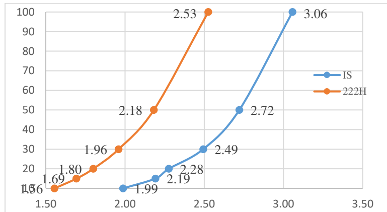
Fig. 2.2: Design Wind Pressure, kN/m 2 (Face Wind)
