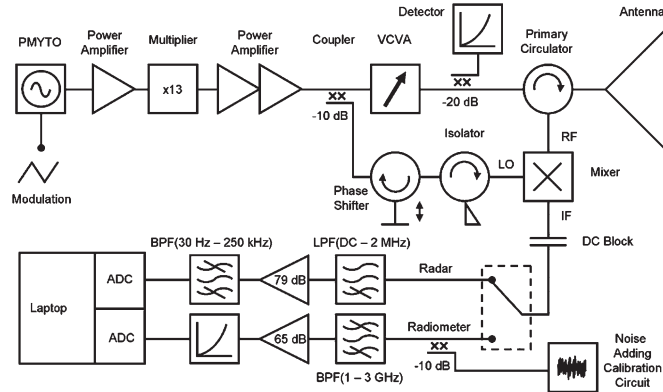
Fig. 2. AVTIS sensor head architecture. The instrument is a heterodyne receiver with radar and radiometer receivers sharing the same mixer. Active and passive measurements cannot be simultaneously performed and are selected by switching the transmit power and receiver chains appropriately.
