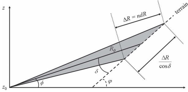
Fig. 14. Geometry of incident radar beam on terrain. The radar is located at z_0 and is usually looking up at an elevation angle \phi onto terrain, which itself has a slope angle \varphi . Application of the low-pass filter in DEM extraction sets an effective footprint size \Delta R , which is n times (integer number of range bins) larger than the spectral resolution of dR . The actual beam intercept on the terrain then depends on the grazing angle \delta .
