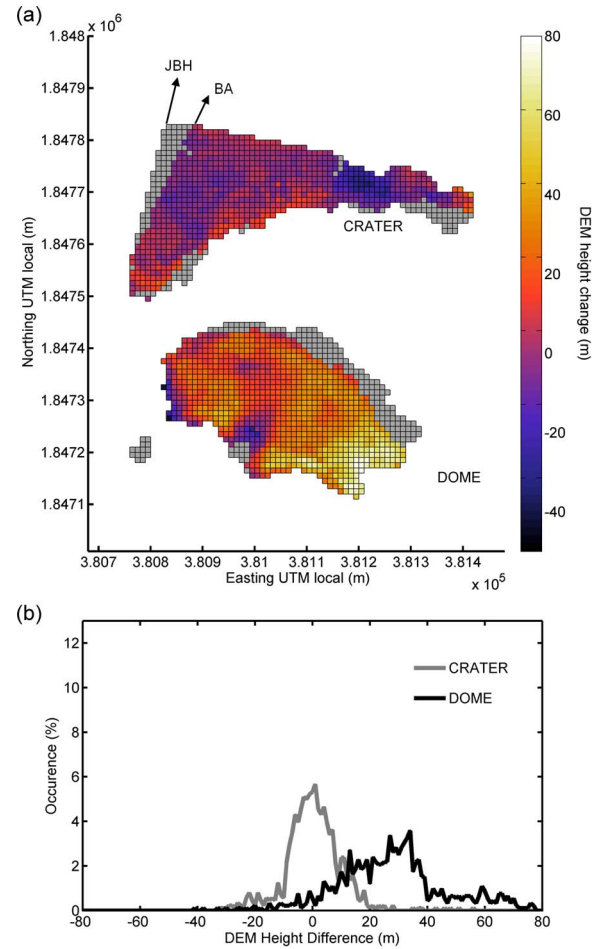
Fig. 19. (a) DEM recorded at a range of \sim 6000 \text{ m} showing dome growth over six days measured from two different locations, Bramble Airport and Jack Boy Hill, April 2006. (b) Histogram of height difference binned at 1-m intervals for the crater and dome regions separately. Topography from two different viewpoints degrades the surface correlation and increases errors in volume change measurement. Note that the scales for both graphs are the same as those in Fig. 18.
