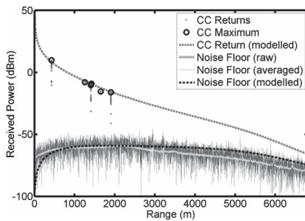
Fig. 13. Data and models characterizing AVTIS radar performance. Maximum reflected power from six fixed CC retroreflectors recorded in the field on Montserrat over a period of two weeks gave a minimum one-way atmospheric loss of 1.3 dB/km. Noise floor data are from clear sky measurements and show good agreement with models based on component specification and laboratory characterization.
