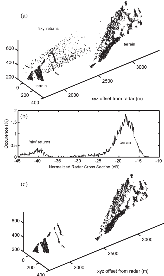
Fig. 7. Three-dimensional topographic point cloud in the radar frame of reference. (a) Topography with spurious “sky” returns corresponding to LOS that do not intercept terrain. (b) Histogram of normalized RCS (RCS per unit area) for the target terrain with points less than -32 dB removed from the data. (c) Topographic point cloud after RCS thresholding.
