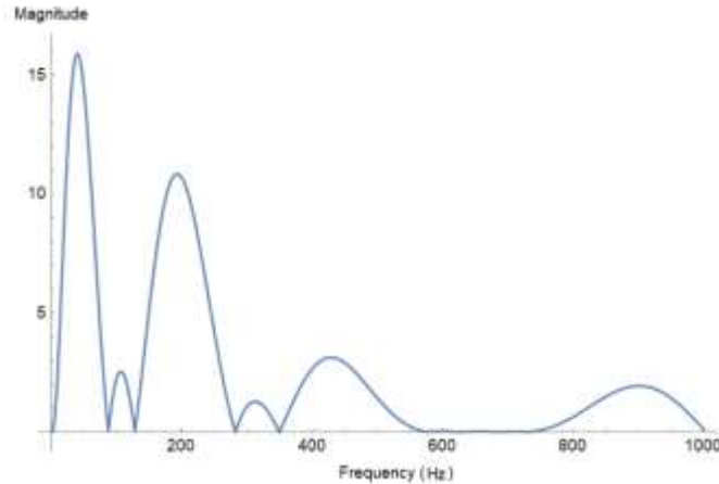
Figure 12: Characteristic polynomial
