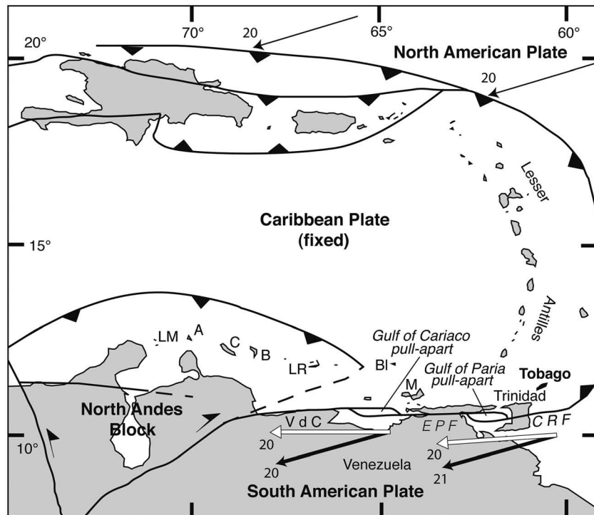
Figure 1. Regional structural geology and plate tectonic setting of the Tobago study area. The Caribbean Plate currently moves ~20 mm/yr eastward relative to South America [Weber et al. , 2001a; DeMets et al. , 2010] along the right-stepping El Pilar (EPF) and Central Range (CRF) strike-slip faults and across associated Gulf of Paria and Gulf of Cariaco pull-apart basins. The Lesser Antilles is a modern arc developing as the Caribbean Plate overrides and subducts Atlantic lithosphere of the North and South American plates. Shown are MORVEL predictions in a fixed-Caribbean reference frame [DeMets et al. , 2010] for Caribbean-South American (thick black arrows) and Caribbean-North American (thin black arrows) relative plate motion vectors (mm/yr). A regional Caribbean-South American plate motion model from Weber et al. [2001a] predicts relative plate motion (white arrows; mm/yr) vectors that are approximately parallel to the E-W azimuth of the El Pilar transform fault. Older oceanic fore-arc and arc crust and lithosphere obducted over and accreted to South American continent crops out mainly as a series of submerged islands including Tobago, Margarita (M), Blanquilla (BI), Los Roques (LR), Bonaire (B), Curacao (C), Aruba (A), and Los Monjes (LM); the Villa de Cura nappe (VdC) is its largest “trapped” on-land exposure.
