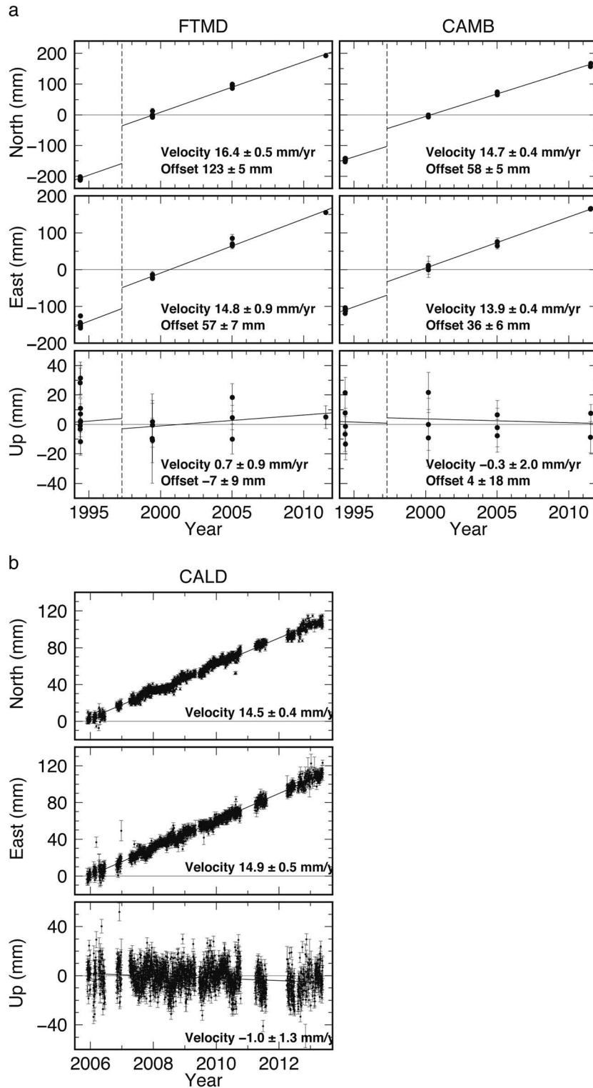
Figure 5. (a) GPS-derived north, east, and up coordinate (dots with error bars) time series for campaign sites 3252, Fort Campbleton (CAMB), in northern Tobago, and 3225, Fort Milford (FTMD), in southern Tobago (see Figure 6), measured before and after the 22 April 1997 Tobago earthquake. Time series are in the ITRF2008 reference frame. Estimated coseismic displacements are labeled as “offset.” All parameters derived used methods described in text. Note that the southern campaign site (FTMD), which is closest to the epicenter, experienced the largest coseismic displacements. (b) Time series for continuous GPS site CALD in central Tobago ( 11.20^\circ , -60.73^\circ ; see Figure 6), also given in ITRF2008. Note that CALD’s east and north interseismic velocity components are very similar to those (labeled as “velocity”) that we estimated for episodic sites CAMB and FTMD.
