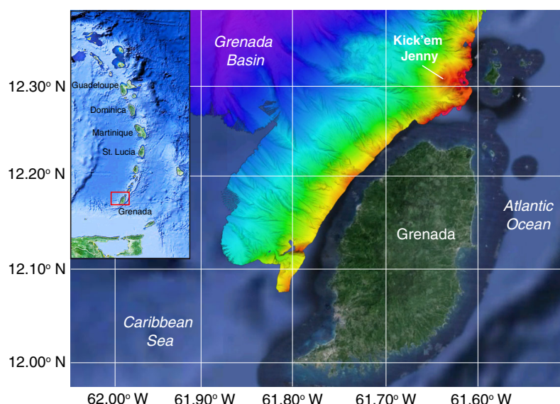
Figure 1. Map showing the location of Kick'em Jenny submarine volcano off the coast of Grenada in the West Indies with shaded multi-beam bathymetry collected during cruise NA-039. Inset map shows the Lesser Antilles island arc and location of the study area (red rectangle).
